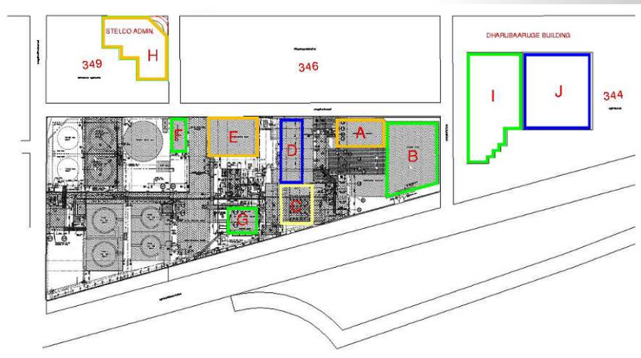
Potential solar collector areas on and close to STELCO power plant
